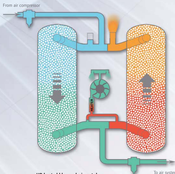
HB heated blower desiccant dryer
